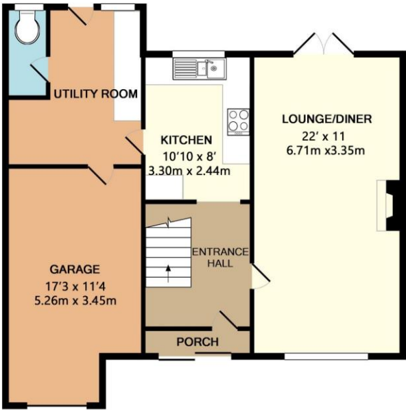
GROUND FLOOR APPROX. FLOOR AREA 689 SQ.FT. (64.0 SQ.M.)
